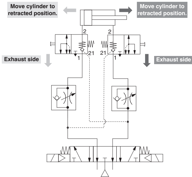
Figure A: Example of piping using exhaust centre valve
