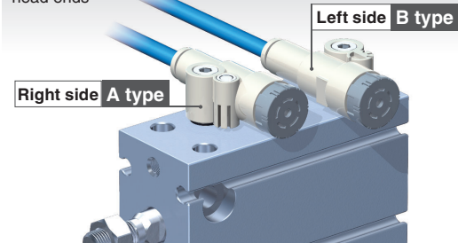
Installation example
