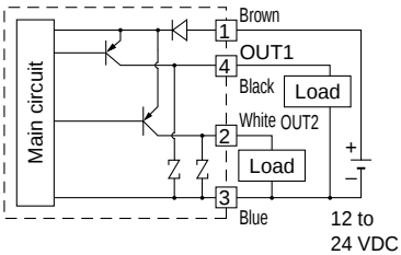
PF2W7□□-□□-67□(-M): PNP type
