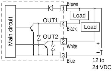
PF2W7□□-□□-27□(-M): NPN type
