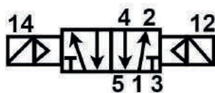
KRB.102 1/4 52 DOUBLE COIL VALVE
